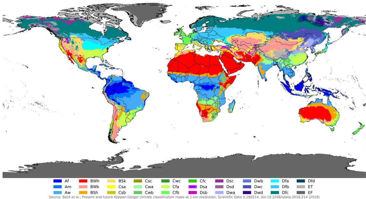
Köppen-Geiger climate classification map (1980-2016)
